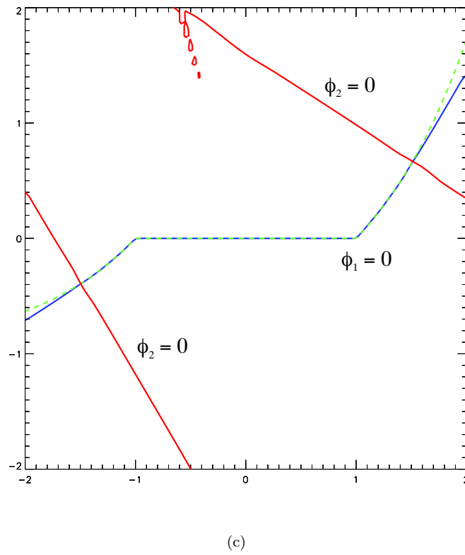
Figure 11. Benchmarking the fast marching algorithm. (a),(b) Exact surface and surface obtained using the FMM algorithm; and (c) Comparison of exact solution and FMM along a cross-section.
