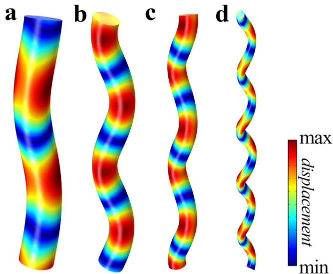
Fig. 7. Buckling modes of fibers in composites with \kappa=15 and v_f = 0.02 (a), 0.01 (b), 0.005 (c) and 0.001 (d). The colors represent the relative in-plane displacement of the points on the surface of buckled fiber from their position in the undeformed fiber.
