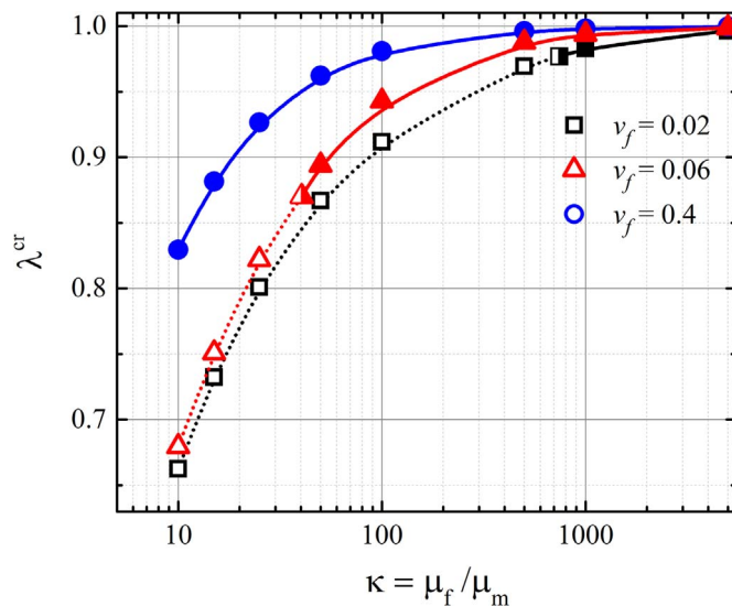
Fig. 5. Dependence of critical stretch ratio \lambda^{cr} on the shear modulus contrast \kappa . Continuous curves and solid symbols correspond to the onsets of macroscopic instabilities, while dotted curves and hollow symbols correspond to the onsets of microscopic instabilities. Half-filled symbols represent the approximate value of \kappa , associated with the transition in the instability modes.
