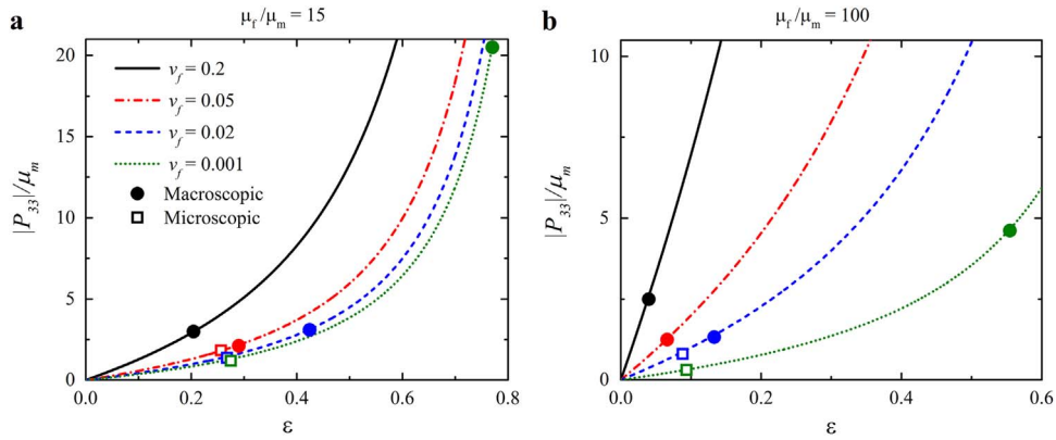
Fig. 3. Stress-strain curves for the fiber composites with \kappa = 15 (a) and \kappa = 100 (b). Circle and square symbols indicate the onsets of macroscopic and microscopic instabilities, respectively.
