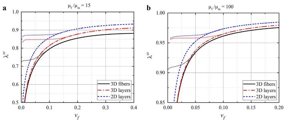
Fig. 9. Dependencies of the macroscopic and microscopic (dotted curves) critical stretch ratios on the volume fraction of rigid phase ( v_f ) for the fiber and layered composites with shear modulus contrasts \kappa=15 (a) and \kappa=100 (b).
