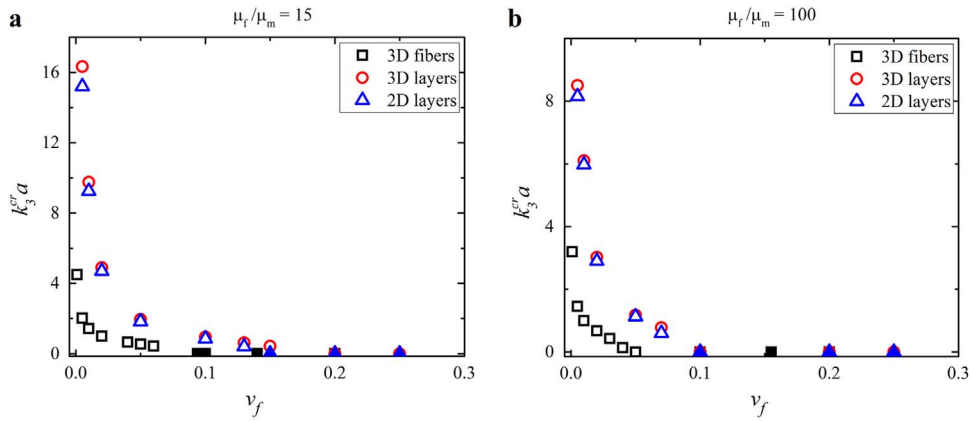
Fig. 10. Dependencies of the critical wavenumber ( k_3^{\text{cr}} ) on the on the volume fraction of rigid phase ( v_f ) for the fiber and layered composites with shear modulus contrasts \kappa=15 (a) and \kappa=100 (b), subjected to different deformation modes.
