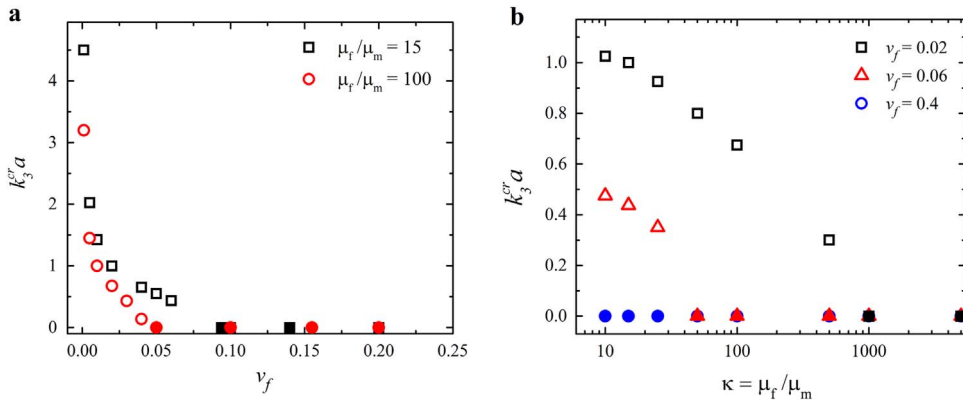
Fig. 6. Dependence of critical wavenumber ( k_3^{cr} ) on the fibers volume fraction v_f (a) and the shear modulus contrast \kappa (b).
