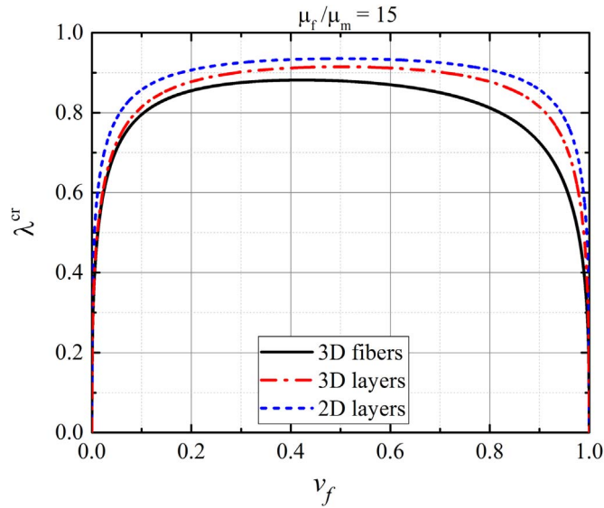
Fig. 8. Dependencies of macroscopic critical stretch ratios on the fibers/layers volume fraction for the fiber (solid black curve) and layered composites (dash-dotted red curve), subjected to uniaxial compression, and layered composites, subjected to compression along the layers direction in plane-strain conditions (blue dashed curve). (For interpretation of the references to color in this figure legend, the reader is referred to the web version of this article.)
