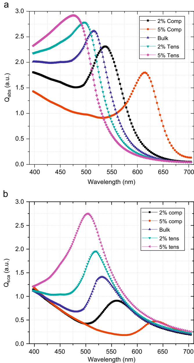
Fig. 1. Plots of (a) absorption (strain-induced Q_{abs} for 100 nm gold nanosphere) and (b) scattering (strain-induced Q_{sca} for 100 nm gold nanosphere) efficiencies for a 100 nm diameter gold nanoparticle as a function of strain.
