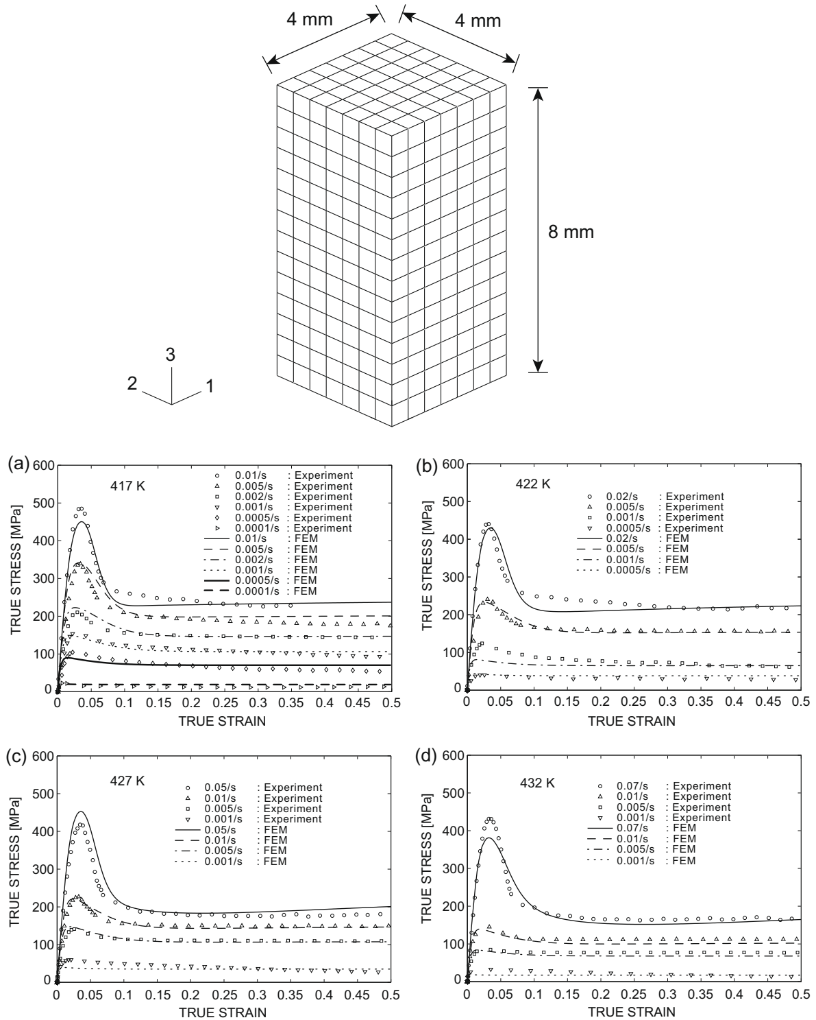
Fig. 3. Initial undeformed mesh of the compression test specimen having dimensions of 4 mm \times 4 mm \times 8 mm, using 686 Abaqus C3D8RT continuum-brick elements. (a) Experimental stress–strain curves in simple compression conducted at ambient test temperatures of (a) 417 K, (b) 422 K, (c) 427 K, and (d) 432 K under a variety of strain rates. Also shown are the predicted stress–strain curves from the coupled thermo-mechanical simulations.
