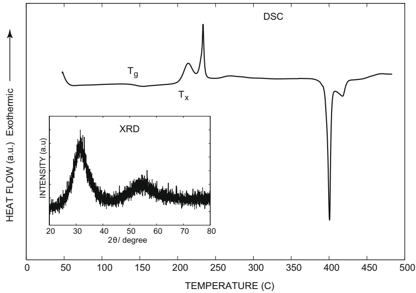
Fig. 1. The DSC data for \text{La}_{61.4}\text{Al}_{15.9}\text{Ni}_{11.35}\text{Cu}_{11.35} amorphous alloy, obtained using a scanning rate of 20^\circ\text{K/min} . The inset represents the XRD pattern for the same alloy, indicating the amorphous nature of the as-cast specimen.
