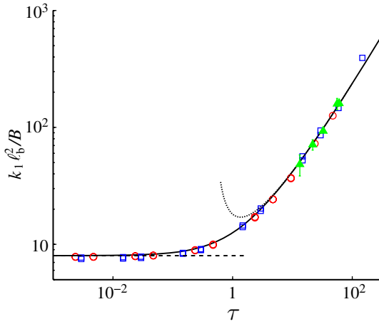
Figure 3. Small indentation. The dependence of the dimensionless shell stiffness k_1 \ell_b^2 / B on the dimensionless pressure \tau , which is defined in equation (3.5). The solid curve shows the theoretical prediction (3.6), which is approximated by the result of Reissner [13], k_1 \sim 8B / \ell_b^2 , for \tau \ll 1 (dashed line) and by equation (3.7) for \tau \gg 1 (dotted curve). Open points show the results from simulations with shell thicknesses h = 2 mm (blue squares) and h = 5 mm (red circles). All other material properties are as in figure 2 a . Solid points (green triangles) show experimental results obtained using a Pezzi ball with error bars given by repeated trials at different loading speeds.
