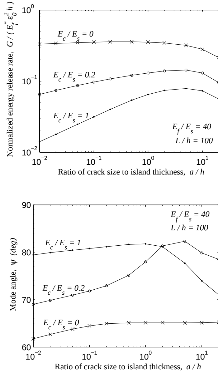
Fig. 4. (a) Normalized energy release rate is plotted as a function of normalized crack size. (b) Mode angle \psi is plotted as a function of normalized crack size.
