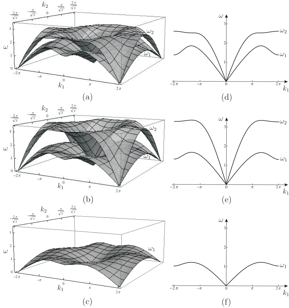
Figure 2: Dispersion surfaces (a-c) and relative cross-sections for k_2 = 0 (d-f) for different values of the spinner constant: \alpha = 0.3 (a,d); \alpha = 0.6 (b,e); \alpha = 2.0 (c,f).
