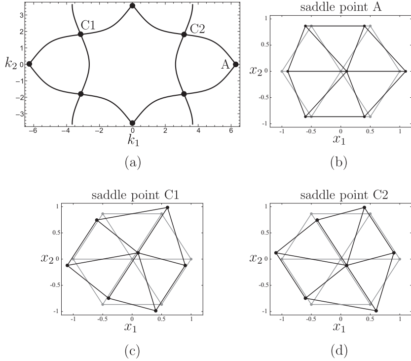
Figure 9: (a) Slowness contour \omega_1 = \sqrt{6/(2 + \sqrt{1 + 3\alpha^2})} for \alpha = 0.9 ; the heavy dots represent the saddle points. (b)-(d) Standing modes at the saddle points A, C1 and C2, specified in (a). The modes (in black) are shown together with the undeformed lattice (in grey).
