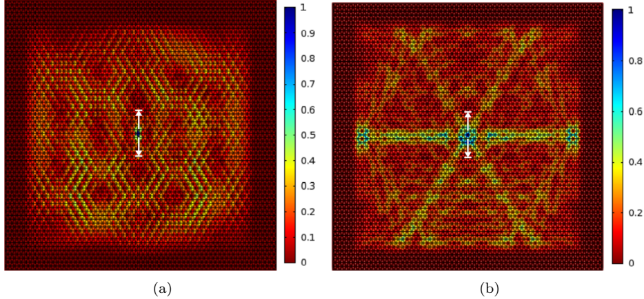
Figure 14: Displacement amplitudes as a result of an applied vertical unit displacement vibrating harmonically at the stationary points frequency \omega = \sqrt{6/(2 - \sqrt{1 + 3\alpha^2})} . The subcritical spinner constants are close to the transition value \alpha = \sqrt{7/27} : (a) \alpha = \sqrt{7/27} - 1/10 ; (b) \alpha = \sqrt{7/27} + 1/10 . (Online version in colour.)
