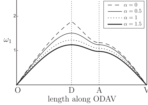
Figure 5: Sections of the lower dispersion surface \omega_1 along the path ODAV, shown in Fig. 4, determined for different values of \alpha .
