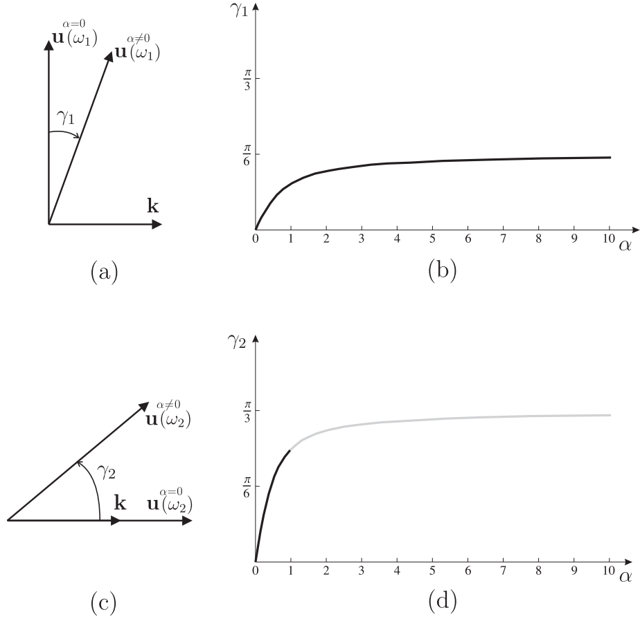
Figure 7: (a) Definition of the angle \gamma_1 ; (b) dependence of \gamma_1 on the spinner constant \alpha ; (c) definition of the angle \gamma_2 ; (d) dependence of \gamma_2 on \alpha , where the grey part of the diagram indicates that waves are evanescent in the supercritical regime \alpha > 1 .
