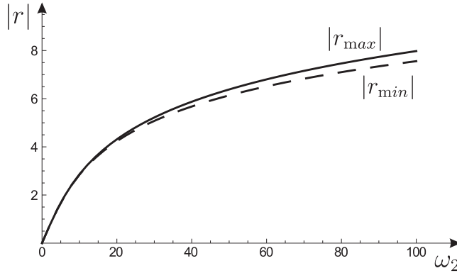
Figure 11: Attenuation coefficient |r| versus frequency \omega_2 for \beta = 0 + n\pi/3 ( |r_{\min}| ) and \beta = \pi/6 + n\pi/3 ( |r_{\max}| ). The curves are given for \epsilon = 0.1 .
