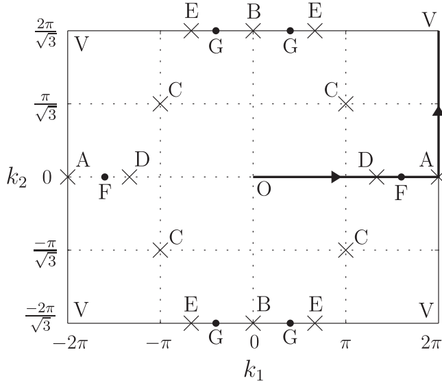
Figure 4: Positions of the stationary points in the k_1 - k_2 plane for \alpha = 0.45 (the crosses indicate fixed points, while the dots represent points moving with \alpha ).
