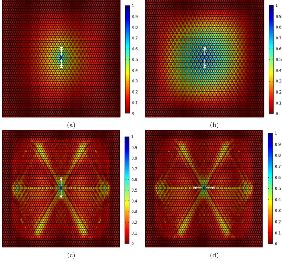
Figure 13: Displacement amplitudes as a result of an applied unit displacement varying harmonically at the stationary points frequency \omega = \sqrt{6/(2 - \sqrt{1 + 3\alpha^2})} (see Table 2, class III). The subcritical spinner constant is: (a) \alpha = 0 ; (b) \alpha = 0.2 ; (c-d) \alpha = 0.9 . (a), (b) and (c) correspond to an applied vertical displacement and (d) to an applied horizontal one. (Online version in colour.)
