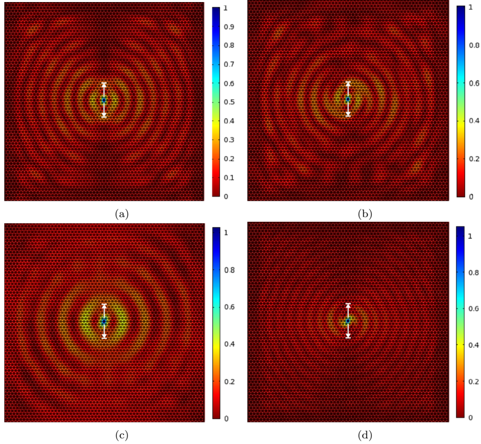
Figure 12: Displacement magnitude fields produced by a vertical harmonic displacement of low frequency \omega = 0.5 , imposed on the central node of the lattice. The displacement fields are given for different values of the spinner constant: (a) \alpha = 0 ; (b) \alpha = 0.5 ; (c) \alpha = 1 ; (d) \alpha = 1.5 . (Online version in colour.)
