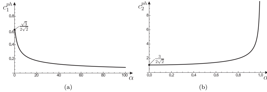
Figure 3: Phase velocities in the neighbourhood of the origin of the irreducible Brillouin zone as a function of the spinner constant \alpha . Results correspond to dispersion surfaces \omega_1 (a) and \omega_2 (b). Note the different ranges of the variables in the two figures.
