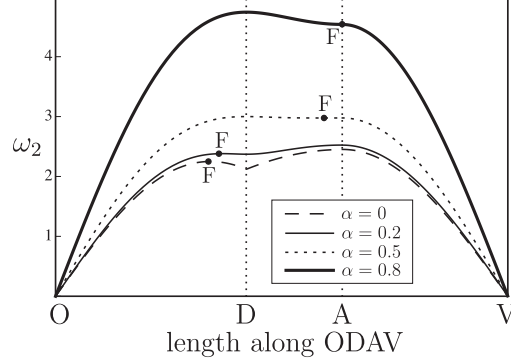
Figure 6: Sections of the upper dispersion surface \omega_2 along the path ODAV, shown in Fig. 4, obtained for different values of \alpha .
