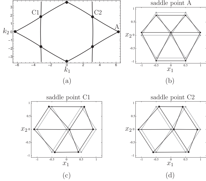
Figure 10: (a) Slowness contour \omega_2 = \sqrt{6/(2 - \sqrt{1 + 3\alpha^2})} for \alpha = 0.9 ; the saddle points at this frequency are indicated by heavy dots. (b)-(d) Standing modes at the saddle points A, C1 and C2, specified in (a). The modes (in black) are shown together with the undeformed lattice (in grey).
