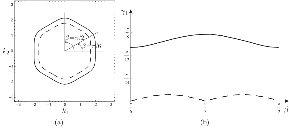
Figure 8: (a) Slowness contours \omega_1(\mathbf{k}) = 1 , obtained for \alpha = 0.9 (solid line) and \alpha = 0 (dashed line); (b) relations between polarisation angle \gamma_1 and wave vector angle \beta for \alpha = 0.9 (solid line) and \alpha = 0 (dashed line), evaluated in the sector \pi/6 \leq \beta \leq \pi/2 .
