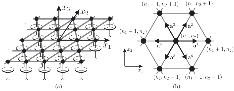
Figure 1: (a) Monatomic triangular lattice, connected to a system of gyroscopes; (b) plane representation of a lattice cell.
