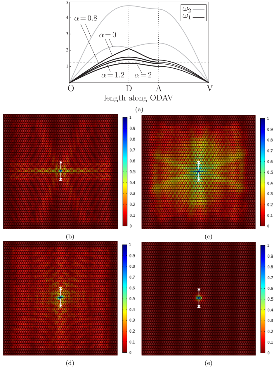
Figure 15: (a) Dispersion curves \omega_1 (in black) and \omega_2 (in grey) along the path ODAV indicated in Fig. 4. The curves are given for spinner constant \alpha = 0, 0.8, 1.2, 2.0 corresponding to part (b-e) of the figure, respectively. (b-e) Displacement amplitudes in the chiral lattice as a result of an applied vertical unit displacement at frequency \omega = 1.27 , represented in part (a) with a dashed line. (Online version in colour.)
