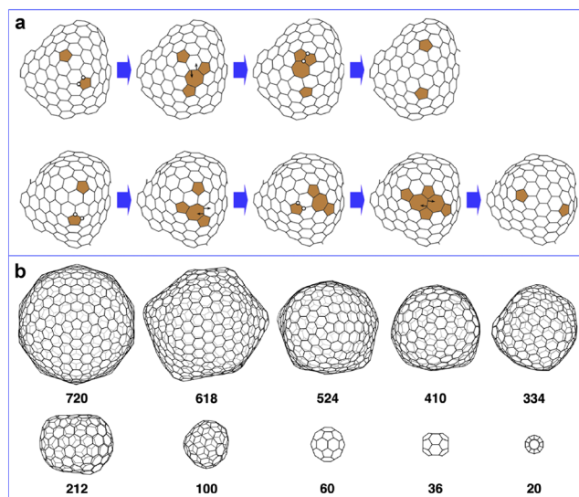
FIG. 4 (color online). Typical C_2 removal process and the annihilation of 5|7 defects in the large fullerene surface [(a), upper panel] and snapshots of the shrinking of fullerenes during the simulation process [(b), lower panel].
