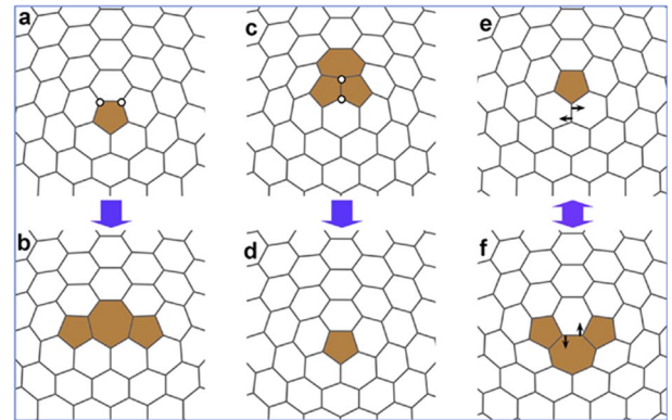
FIG. 3 (color online). A pentagon acts as both a source and a sink of a 5|7. (a), (b) Removal of a C_2 from a pentagon creates a 5 + 5|7 defect; (c), (d) when a 5|7 approaches to a pentagon, removal of a C_2 annihilates the 5|7 defect; (e), (f) a bond rotation step annihilates a 5|7 in the vicinity of a pentagon, and the reverse process creates an additional 5|7.
