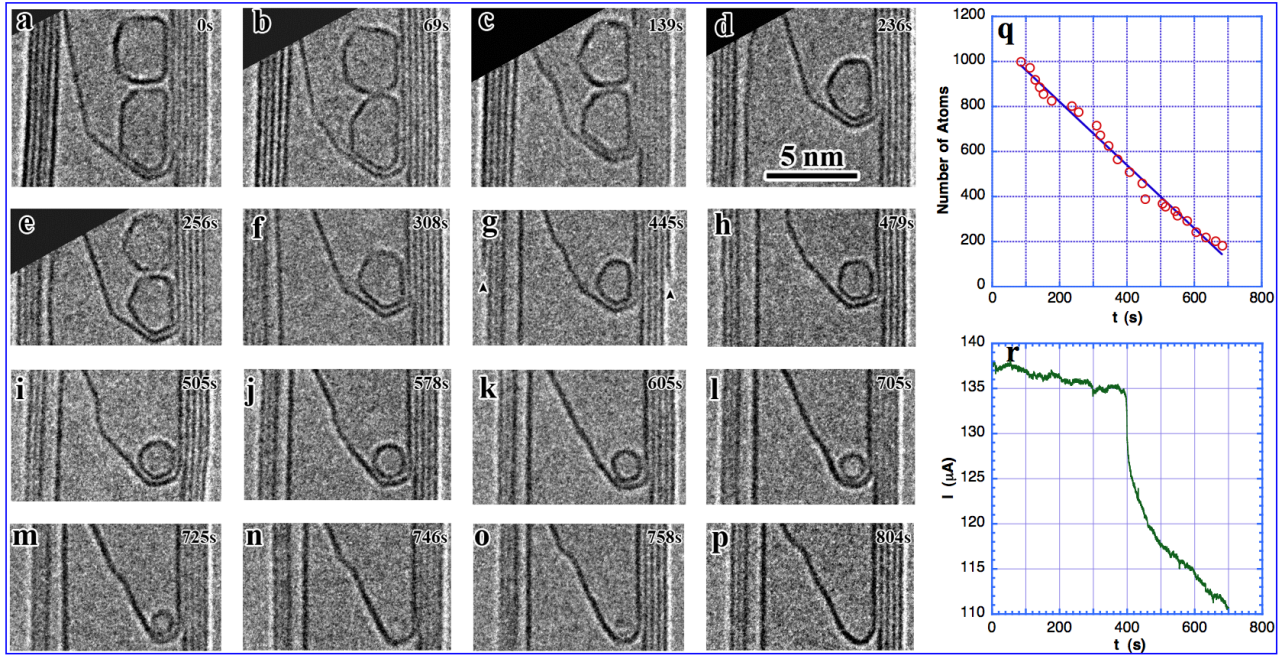
FIG. 1 (color online). (a)–(p) Continuous shrinkage of a giant fullerene ( C_{1300} ) trapped inside the cavity of a MWCNT at high temperatures. The time elapse (in seconds) are marked in the figure. Note the outer diameter of the MWCNT is reduced from 9.6 nm in (a) to 9.2 nm in (p) due to evaporation of carbon atoms. (q) The number of carbon atoms in the fullerenes decrease linearly with time during the sublimation process; (r) the bias voltage in the MWCNT remains constant at 2.26 V and the current is reduced from 137 \mu A to 110 \mu A during the fullerene shrinkage process. Note that there is a sharp current drop of about 10 \mu A at t = 400 s, which is caused by the breakdown of the outmost shell [marked by two upper-pointed arrowheads in (g)]. The slow current drop is caused by the diameter reduction and defects in the MWCNT.
