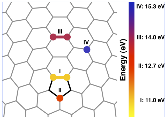
FIG. 2 (color online). Energy cost of removing a C_2 and a C_1 from different sites in the fullerene C_{320} .
