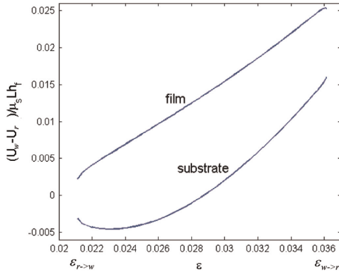
Fig. 11. The elastic energy differences between the wrinkle state and ridge state U_w - U_r in the film (top curve) and substrate (bottom curve) in the strain range \varepsilon_{r \rightarrow w} < \varepsilon < \varepsilon_{w \rightarrow r} , with \mu_f/\mu_s = 1000 , (h_f + h_s)/h_f = 200 , \lambda_0 = 2 and period L = 9h_w .
