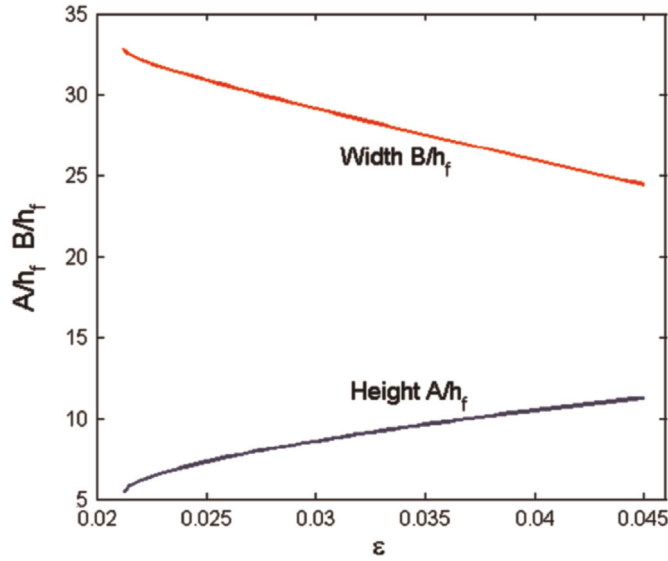
Fig. 10. The variation of the normalized width B and height A of the ridge (cf., Fig. 2e) as a function of strain \varepsilon for \mu_f/\mu_s = 1000 , (h_f + h_s)/h_f = 200 , \lambda_0 = 2 and period L = 9h_w .
