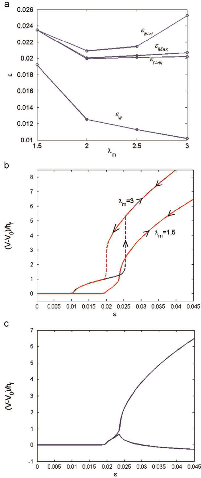
Fig. 13. The influence of the strain-stiffening effect on the formation of ridges. (a) The dependence of the strain at the onset of wrinkling \varepsilon_w , the two transition strains, and the Maxwell strain for ridges on the limit stretch of the substrate \lambda_m , with the substrate modeled as an Arruda-Boyce material. (b) The vertical displacement relative to the displacement under uniform deformation V - V_0 of the ridge peak as a function of strain \varepsilon during loading and unloading for \lambda_m = 3 and 1.5 . The loading and unloading shows no hysteresis for \lambda_m = 1.5 . (c) The relative vertical displacements V - V_0 of the ridge peak and its neighboring wrinkle peak as a function of strain \varepsilon for \lambda_m = 1.5 , illustrating the onset of ridge localization and the absence of hysteresis. For all the simulations, the other parameters are set as \mu_f/\mu_s = 1000 , (h_f + h_s)/h_f = 200 , \lambda_0 = 2 and period L = 9\lambda_w .
