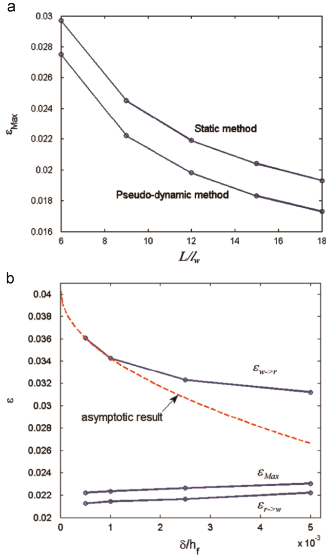
Fig. 8. (a) Effect of the solution periodicity L/h_w on the Maxwell strain \epsilon_{Max} as predicted by the two methods. (b) Effect of the normalized imperfection size \delta/h_f on the transition strains and the Maxwell strain as computed by the pseudo-dynamic method. The wrinkle to ridge transition is highly imperfection-sensitive because the perfect system has an asymmetric bifurcation. The asymptotic relation for sufficiently small imperfections is shown, determined as discussed in the text. The simulation results are for pre-stretch \lambda_0 = 2 , modulus ratio \mu_f/\mu_b = 1000 , thickness ratio (h_f + h_b)/h_f = 200 and period L = 9h_w .
