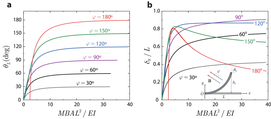
Fig. 6. Free-end location of the deflected elastica plotted against the normalized magnetic field strength MBAL^2/EI with various angles \varphi : (a) angular displacement \theta_L ; (b) normalized tip deflection \delta_y/L .
