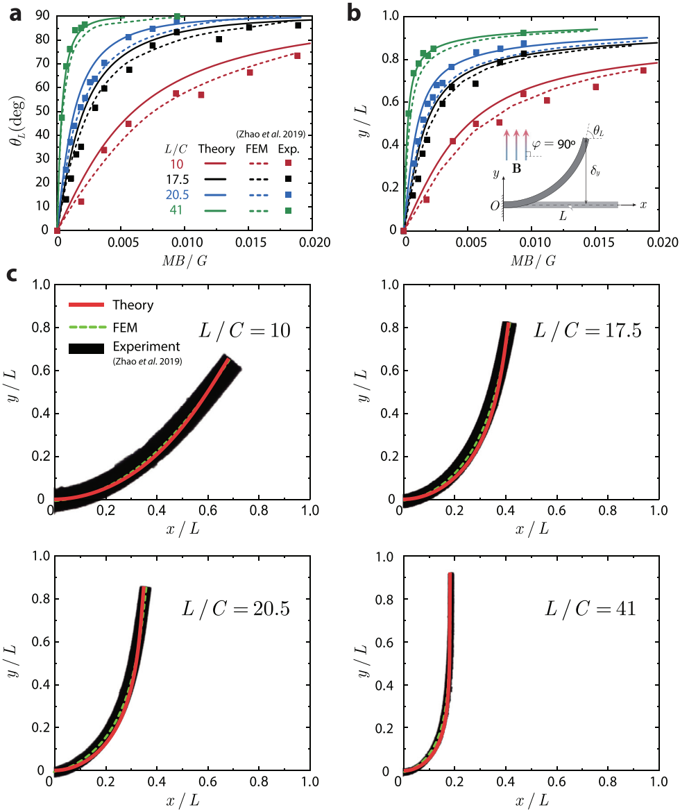
Fig. 7. Comparison of our analytical predictions from the developed hard-magnetic elastica theory with finite element simulation (FEM) and experimental results (Zhao et al., 2019) under a perpendicular magnetic field ( \varphi = 90^\circ ). (a)-(b) The tip rotation angle \theta_L and normalized tip deflection \delta_y/L plotted each as a function of the normalized magnetic flux density MB/G . The inset shows the schematic of the hard-magnetic elastica under consideration. (c) Deformed elastica with different length-to-thickness ratios L/C = 10, 17.5, 20.5, 41 . The black shapes are experimental observations, and the dashed lines and red curves represent the centerlines of the deformed beam predicted from FEM simulations and analytical solutions. The applied magnetic field strength ranges from 0 to 50 mT, which corresponds to the normalized magnetic field strength MB/G ranging from 0 to 0.0019.
