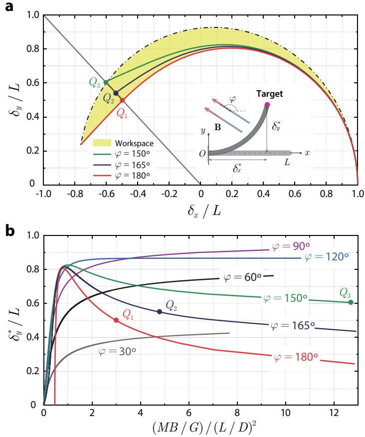
Fig. 10. The control variables ( \varphi, B, L ) required for the robot's end effector to reach a target location ( \delta_x^*, \delta_y^* ) can be determined from the workspace analysis. (a) The required magnetic field direction \varphi can be identified from the intersection between the straight line with a slope of \delta_y^*/\delta_x^* and the tip trajectory in the workspace. (b) Target deflection \delta_y^*/L plotted against the normalized magnetic field input (MB/G)/(L/D)^2 .
