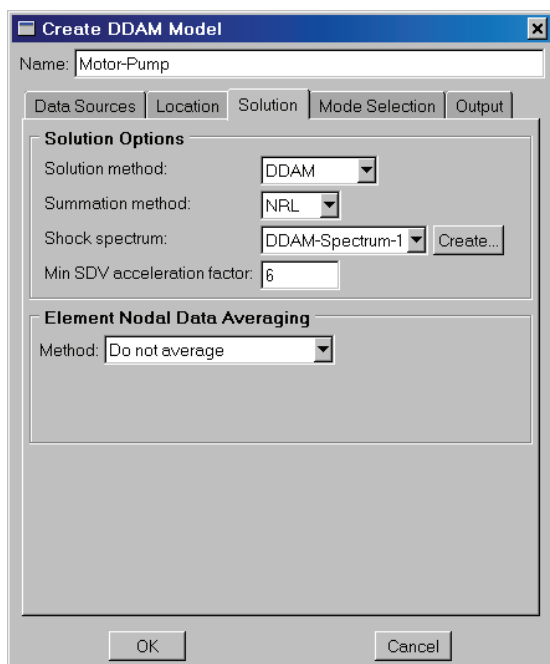
Figure 5: Specification of solution options.
