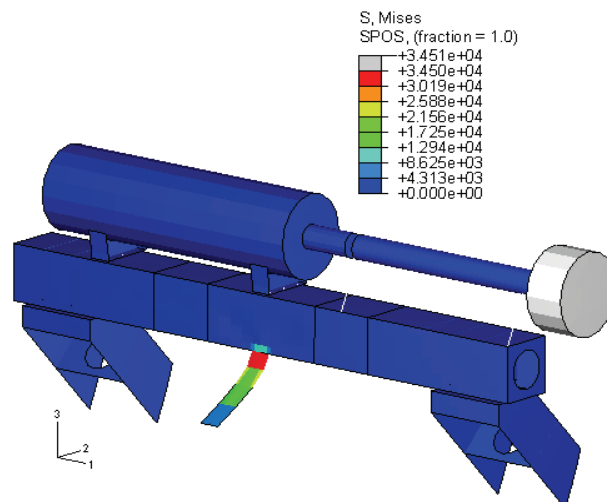
Figure 16: Peak Mises stress response in mode 12.
