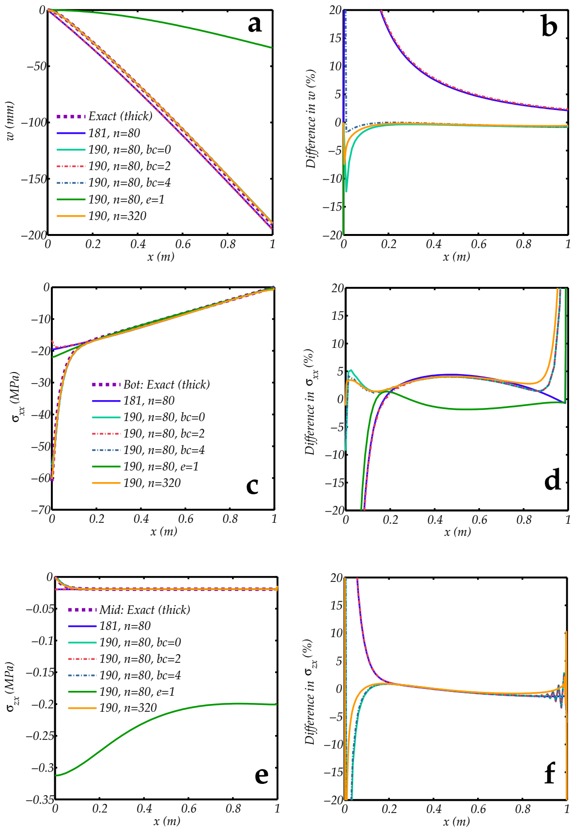
Figure 24 – Displacement and stresses in the thin cantilever sandwich plate under concentrated edge load modeled with SOLSH190 elements. The “exact” solution is the thick-facesheet approximation. The SHELL181 solution with 80 elements along an edge has also been shown for comparison.
