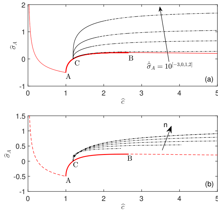
Figure 5. (a) Unloading curves of the dimpled surface starting from \hat{\sigma}_A = 0 for \alpha_d = 0.5 , n = 0.5 and \dot{\hat{\sigma}}_A = 10^{[-3,0,1,2]} . Red lines for the Griffith elastic solution, dot-dashed black lines for the a rate-dependent unloading curves. (b) As panel (a) but for \dot{\hat{\sigma}}_A = 1 and n = [0.1, 0.3, 0.5, 0.7, 0.9] .
