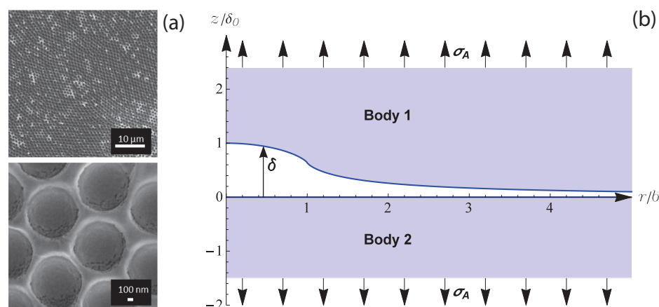
Figure 1. (a) SEM images of a surface patterned with dimples (adapted from [9]). (b) Geometry of the dimple surface considered in this study. The model is axysymmetric.
