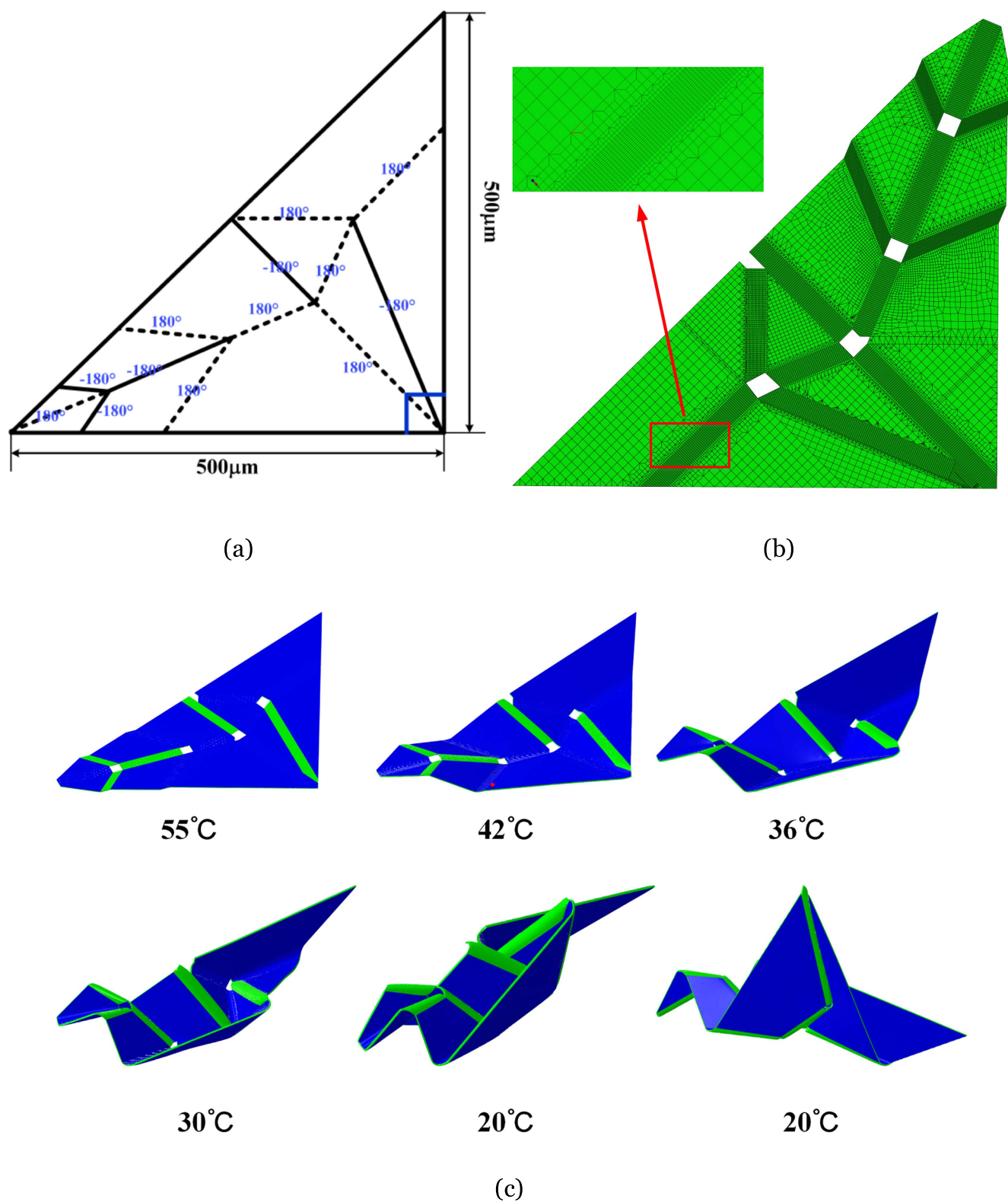
Figure 3. Self-folding of the Randlett's flapping bird. (a) The design of a trilayer film patterned to fold into a Randlett's bird. All open stripe widths are set to be 30\mu\text{m} , such that all the foldings are 180^\circ . The solid lines and the dashed lines represent the locations of mountain and valley folds, entailing controllable folding processes and programmable shape selections. (b) FE Mesh and detailed mesh transition. Mesh refinement is needed along the folding creases as shown by the manifested local view. (c) Folding configurations of the Randlett's bird as temperature varied from 55^\circ\text{C} to 20^\circ\text{C} , numerically reproducing the experiment reported in [22].
