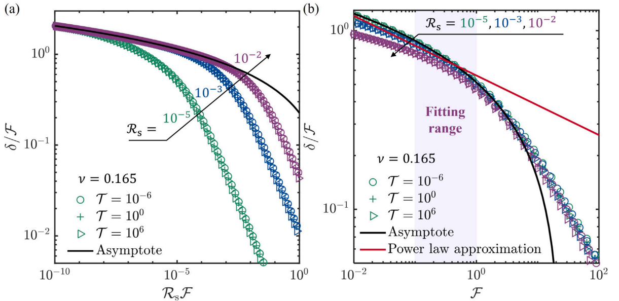
Fig. 9. (a) \delta/F vs. R_s F for various R_s and shear numbers \tau . The asymptotic solutions are given by Eq. (29) when F \ll R_s \ll 1 . (b) \delta/F vs. F for various R_s and shear numbers \tau . The asymptotic solutions are given by Eq. (29) when R_s \ll F \ll 1 . The approximate solutions, given by Eq. (30), are obtained through power law fitting of the numerical data (indicated by markers) within the fitting range indicated by the purple background.
