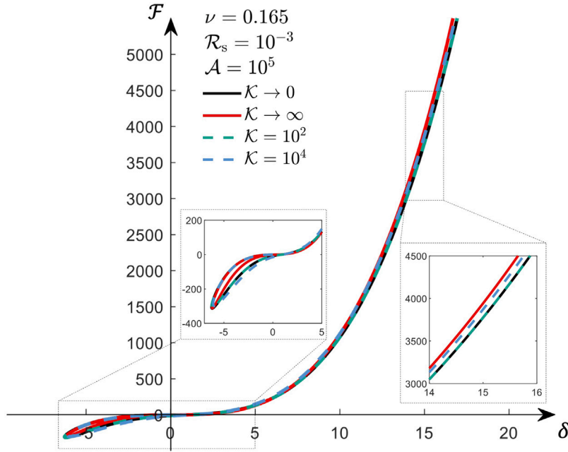
Fig. 6. F vs. \delta for various friction numbers \mathcal{K} when \mathcal{R}_s = 10^{-3} and \mathcal{A} = 10^5 are fixed.
