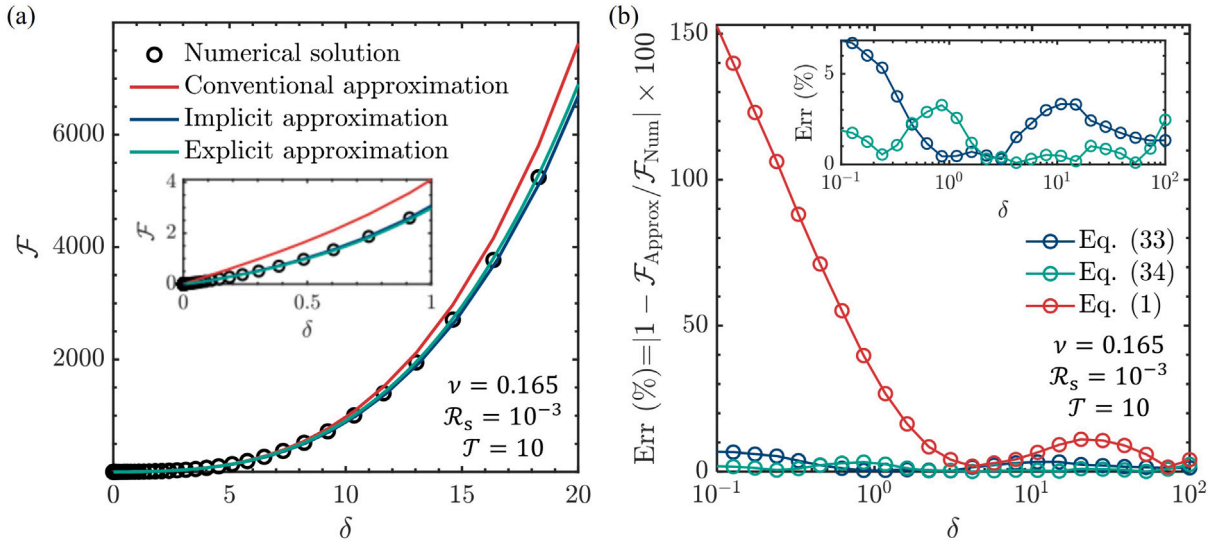
Fig. 12. (a) F vs. \delta obtained from numerical solutions, Eq. (1) (Schwerin-type approximation), Eq. (33) (our implicit approximation), and Eq. (34) (our explicit approximation) when R_s = 10^{-3} and T = 10 . (b) Comparison of the errors of the three approximations relative to the numerical solutions.
