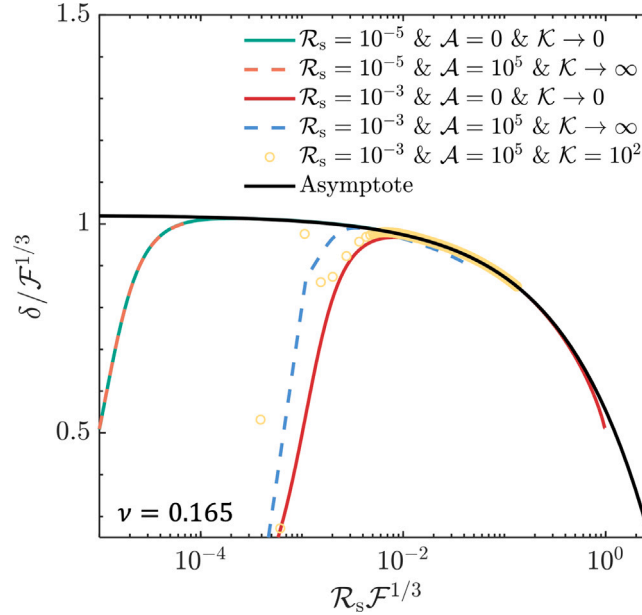
Fig. B.4. \delta / \mathcal{F}^{1/3} vs. \mathcal{R}_s \mathcal{F}^{1/3} under various \mathcal{R}_s when considering a fixed edge and two types of tip/membrane contacts: the non-adhesive and frictionless contact ( \mathcal{A} = 0 & \mathcal{K} \rightarrow 0 ) and the adhesive and non-slip contact ( \mathcal{A} = 10^5 & \mathcal{K} \rightarrow \infty ). The asymptotic solutions are given by Eq. (31) at \mathcal{T} \rightarrow \infty (i.e., the asymptote for drumhead nanoindentation with a fixed edge using a non-adhesive and frictionless spherical tip of finite radius).
