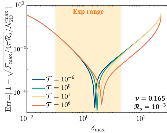
Fig. 13. The error (Err) in the maximum membrane stress induced by Eq. (2) relative to the numerical solutions for varying \tau when R_s = 10^{-3} is fixed.
