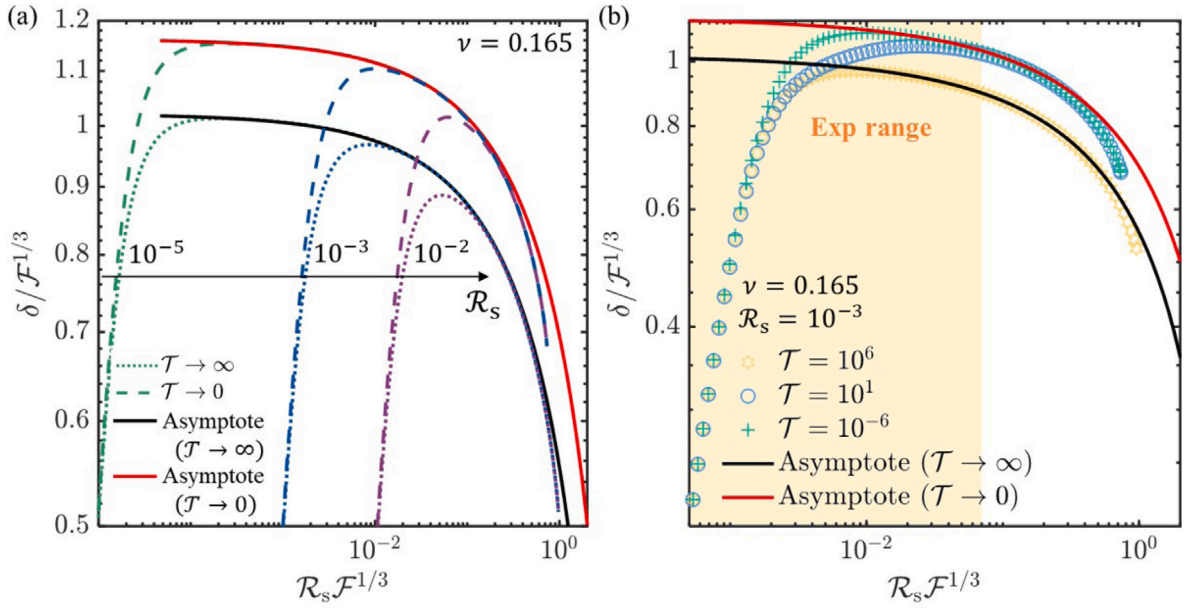
Fig. 10. (a) \delta/F^{1/3} vs. R_s F^{1/3} for various R_s at the two limits: the fixed edge ( T \rightarrow \infty ) (black) and the frictionless edge ( T \rightarrow 0 ) (red). (b) \delta/F^{1/3} vs. R_s F^{1/3} for various T when R_s = 10^{-3} . Here, the asymptotic solutions to the two limiting cases are given by Eq. (31).
