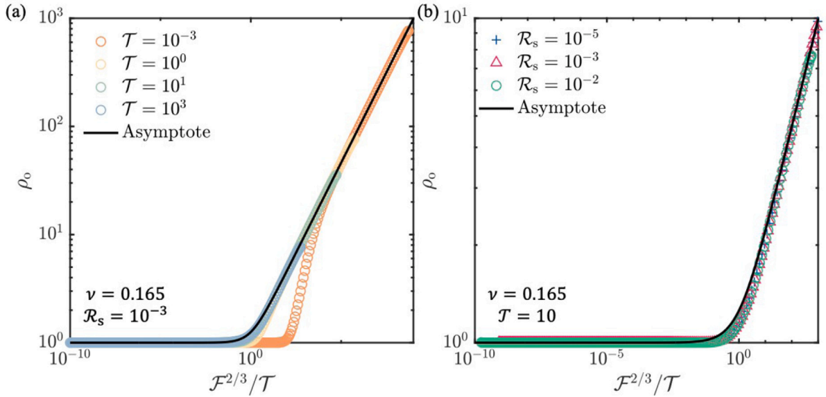
Fig. 11. The dimensionless size of the shear zone, \rho_o , vs. F^{2/3}/T for (a) various T when R_s = 10^{-3} , and (b) various R_s when T = 10 . The asymptotic solutions are given by Eq. (32).
