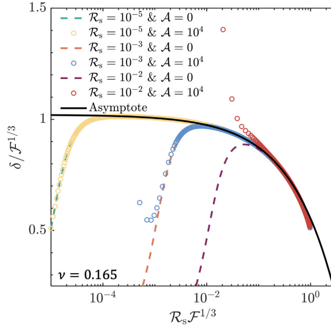
Fig. B.1. \delta/F^{1/3} vs. R_s F^{1/3} under various R_s and A . The asymptotic solutions are given by Eq. (31) at \mathcal{T} \rightarrow \infty (i.e., the asymptote for drumhead nanoindentation with a fixed edge using a non-adhesive and frictionless spherical tip of finite radius).
