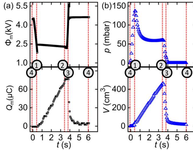
Figure 3. Time evolution of work-conjugate variables during one full conversion cycle. (a) Voltage \Phi_m (top) and charge Q_m (bottom) on the membrane. (b) Excess pressure p (top) and volume V (bottom) of the balloon. Dashed red lines with number labels correspond to the respective states in Fig. 2.
