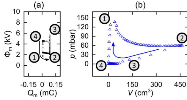
Figure 4. Measured cycle depicted in the (a) electrical and (b) mechanical work-conjugate plane. The areas enclosed by the contours correspond to (a) the generated electrical energy ( 156 \text{ mJ} \hat{=} 102 \text{ mJ/g} ) and (b) the used mechanical energy ( 2.08 \text{ J} \hat{=} 1.36 \text{ J/g} ).
