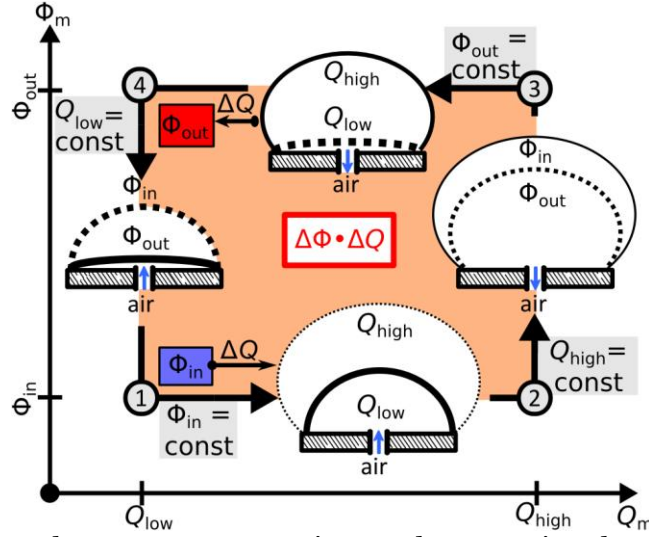
Figure 2. Rectangular energy conversion cycle operating between two charge reservoirs depicted in the work-conjugate (\Phi, Q) plane. The cycle proceeds counter-clockwise from state 1 to state 4. During the four steps of the cycle solid and dashed lines indicate the evolution of the balloon shape. In the constant voltage steps, 1 \rightarrow 2 and 3 \rightarrow 4 , charges are taken from the low voltage reservoir and fed into the high voltage reservoir. In the constant charge steps 2 \rightarrow 3 and 4 \rightarrow 1 , the voltage across the membrane is brought in line with the reservoirs. The area enclosed by the contour corresponds to the generated electrical energy \Delta\Phi\Delta Q .
